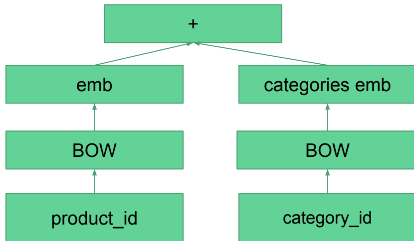
context embedding
