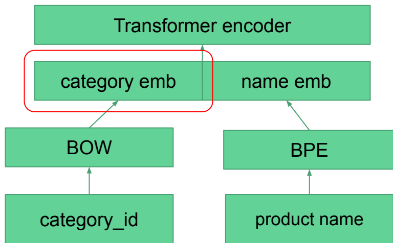
center embedding
